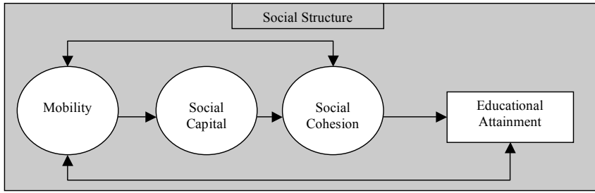
Figure 9.1: Conceptual Model
